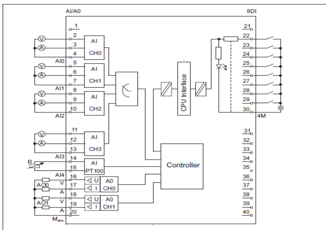
Figure 7-6 Block diagram of integrated digital/analog I/O of CPUs 313C/314C-2
