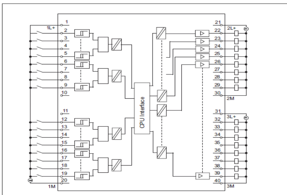
Figure 7-4 Block diagram of integrated digital I/O of CPUs 313C/313C-2/314C-2
